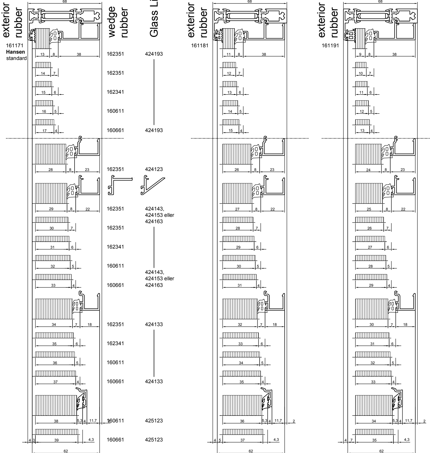
G30 glass entry overview Fixed field, 7 mm ext.
